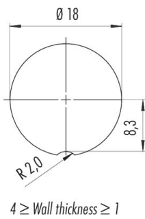
With nose as anti-rotation device
