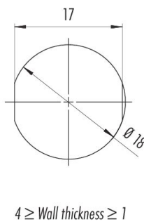
With flats as anti-rotation device
